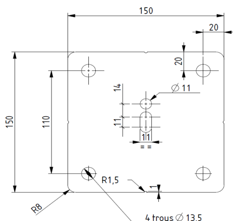
Dimension platine
