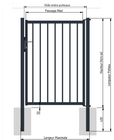
Version 1 vantail
